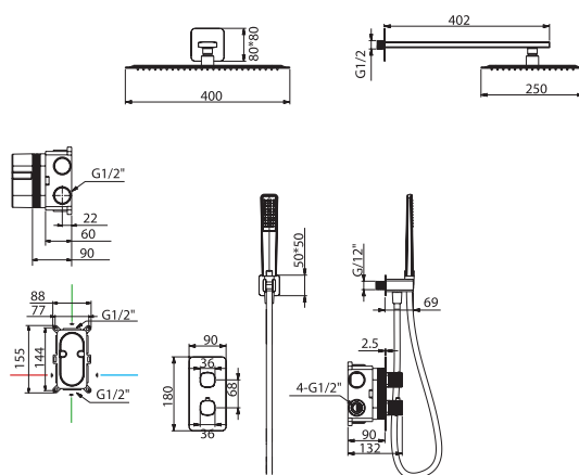
Single-lever 1 way concealed shower - showerhead.
